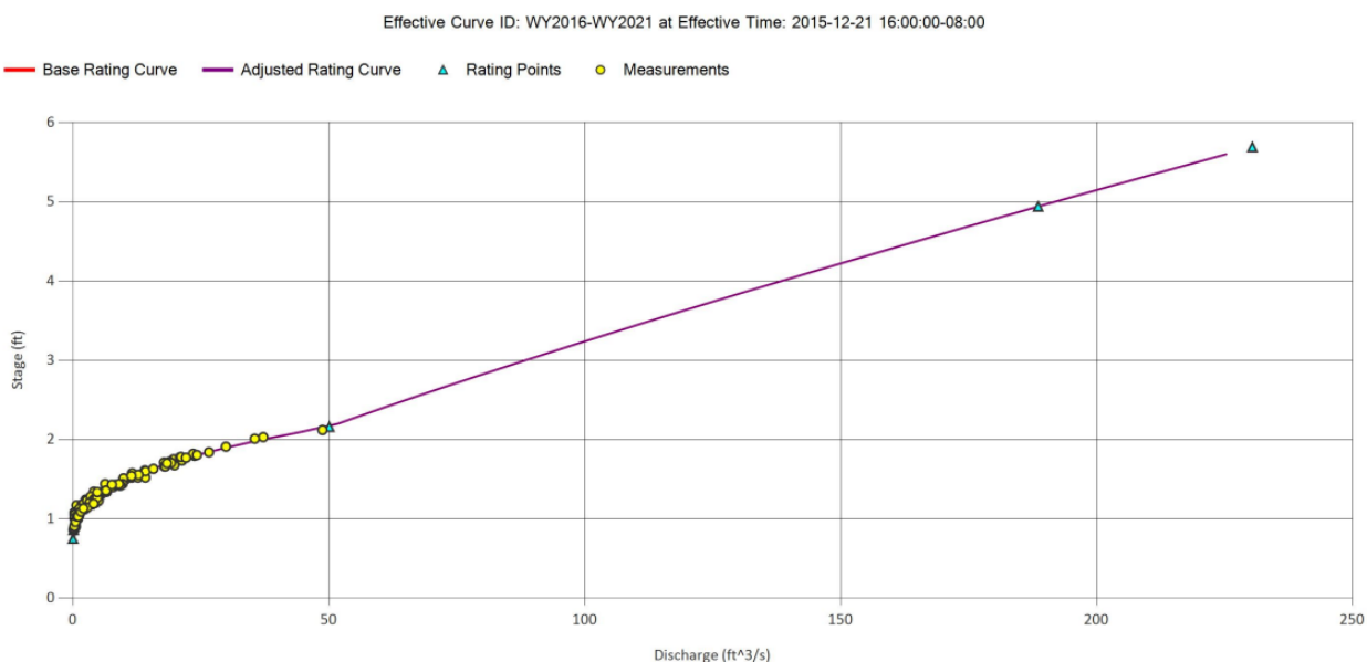
Figure 3. Discharge-stage relationship used for the 2021 WY.
