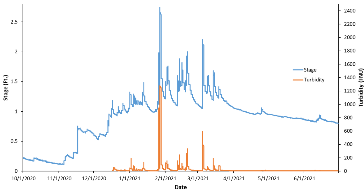
Figure 8. Continuous time-series of stage and turbidity at the McCloud Creek TTS station during the 2021 WY.
