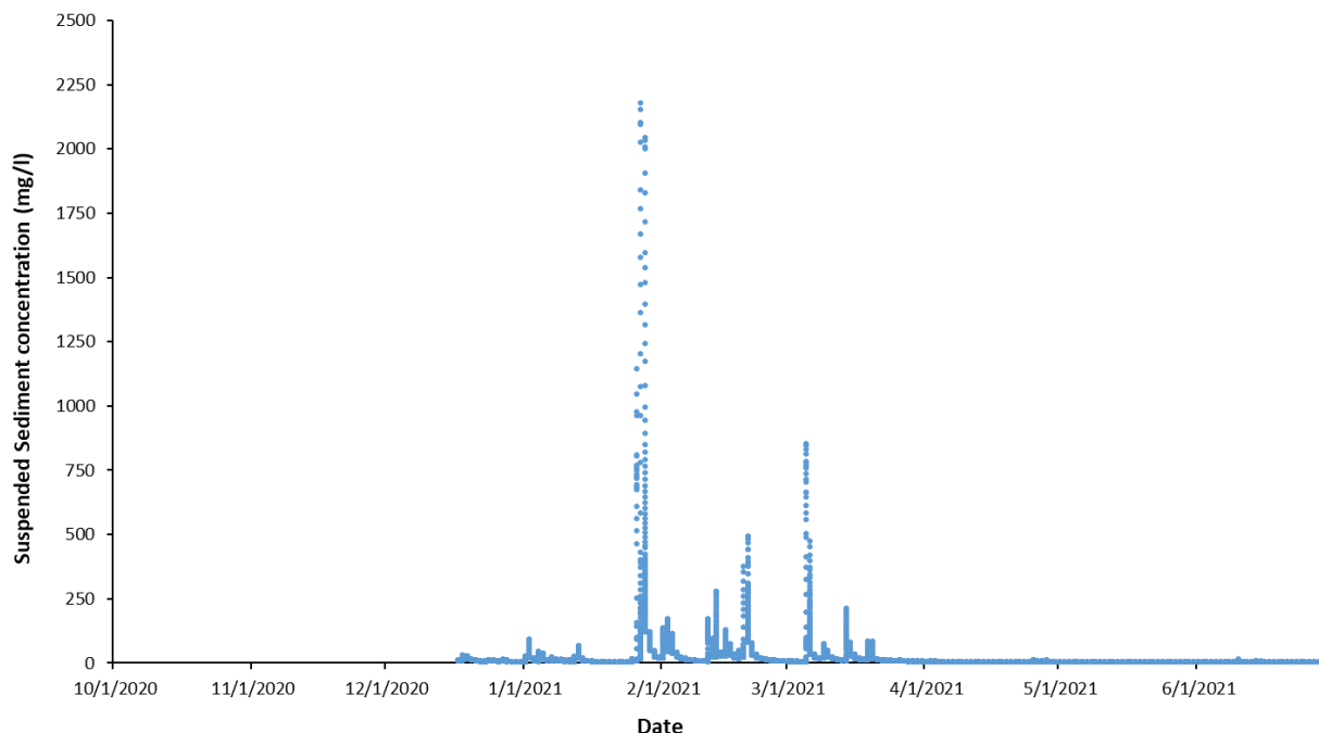
Figure 10. Derived Suspended Sediment Concentration (SSC) based on individual storm's best-fit relationships during the 2021 WY.
