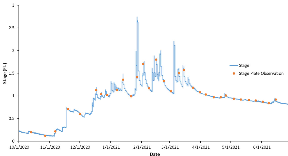
Figure 2. Continuous Time-Series of stage collected by the instream Druck Pressure Transducer sensor and stage plate observations at the McCloud Creek TTS station during the 2021 WY.
