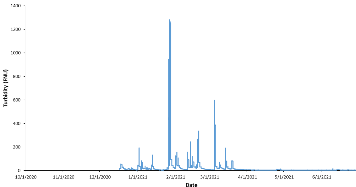
Figure 6. Continuous Time-Series of turbidity collected by the instream DTS-12 sensor at the McCloud Creek TTS station during the 2021 WY.
