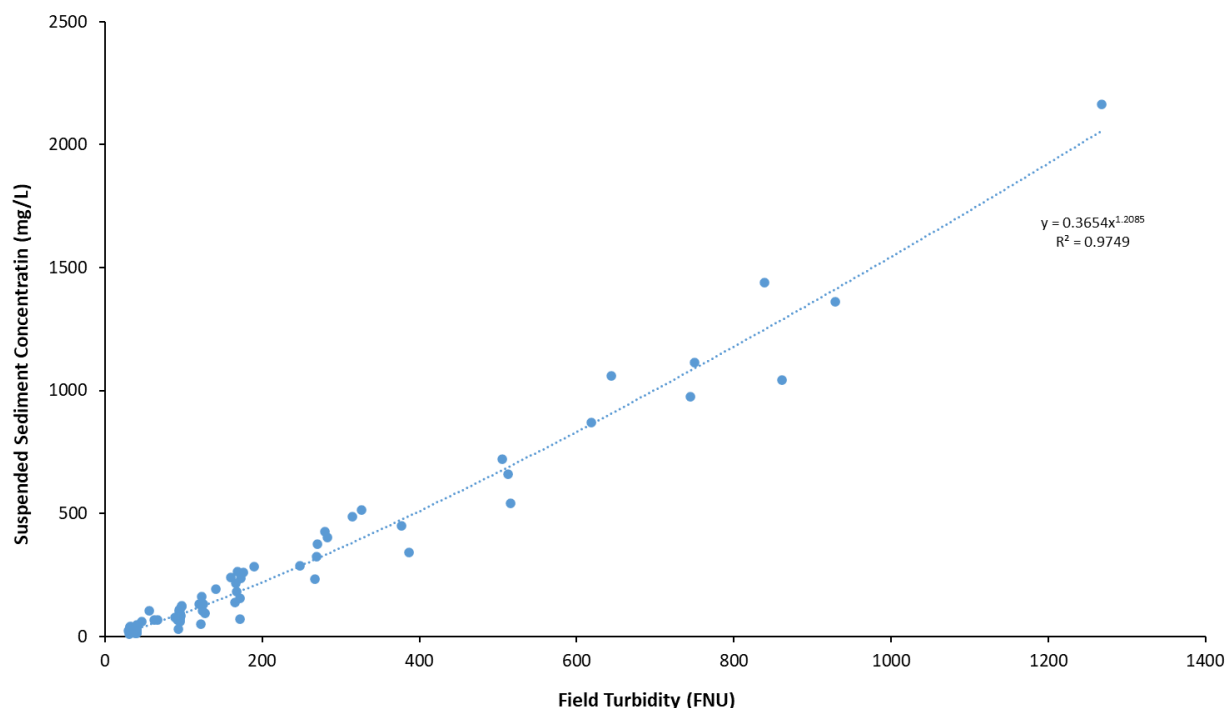
Figure 9. Relationship between turbidity and SSC for the McCloud Creek TTS station during the entire 2021 WY. This graph is an overview of the entire water year.
