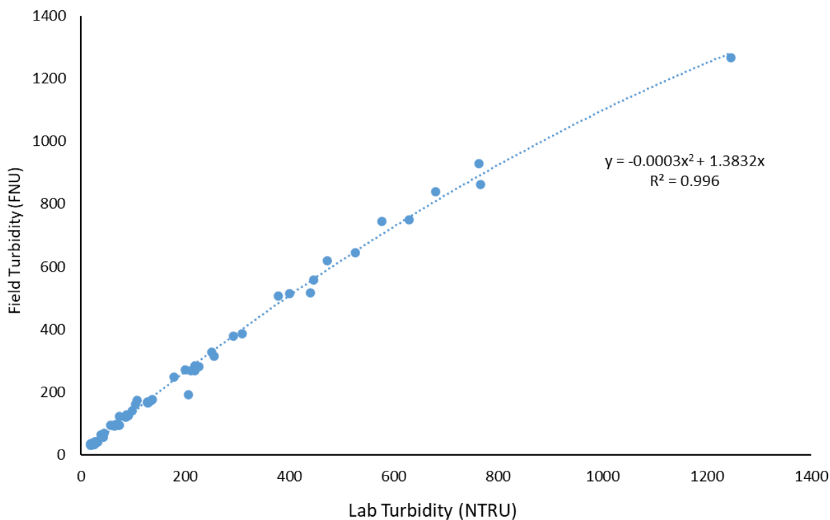
Figure 5. Relationships between coincident field turbidity measurements (FNU) and lab turbidity measurements (NTRU) collected at the McCloud Creek TTS station during the 2021 WY.
