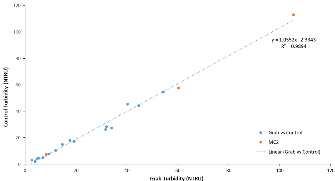
Figure 11. Relationship between turbidity (NTRU) of paired control and grab samples collected across 12 sites during the 2021 WY.
