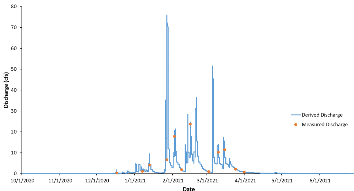
Figure 4. Continuous estimated discharge and measured discharges at the McCloud Creek TTS station during the 2021 WY.
