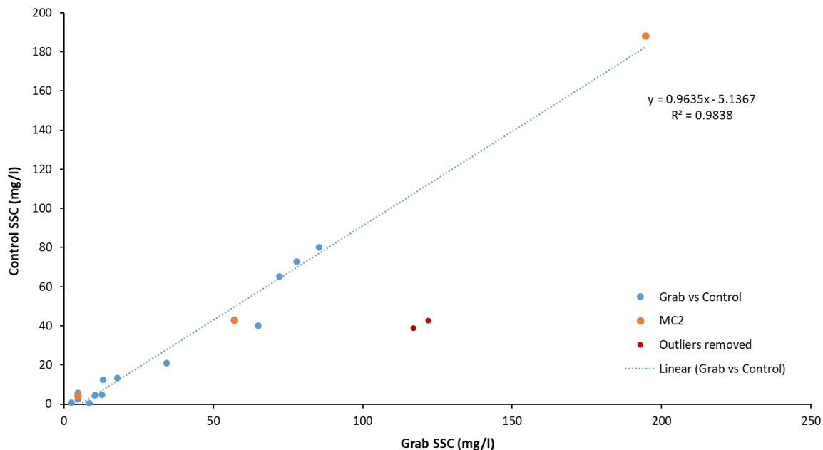
Figure 12. Relationship between suspended sediment concentration (SSC, mg/l) of paired control and grab samples collected across 12 sites during the 2021 WY.
